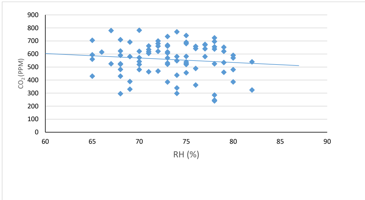
Figure 6: A scatter plot showing the correlation between CO 2 concentration and Relative Humidity (%)
